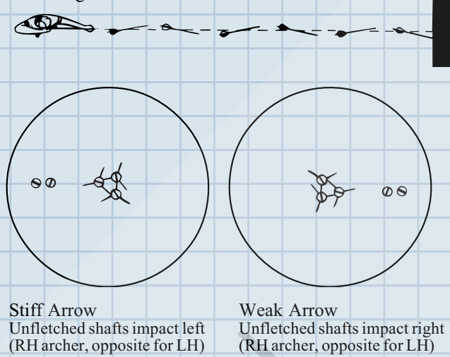
Fig. 11 Fishtailing
