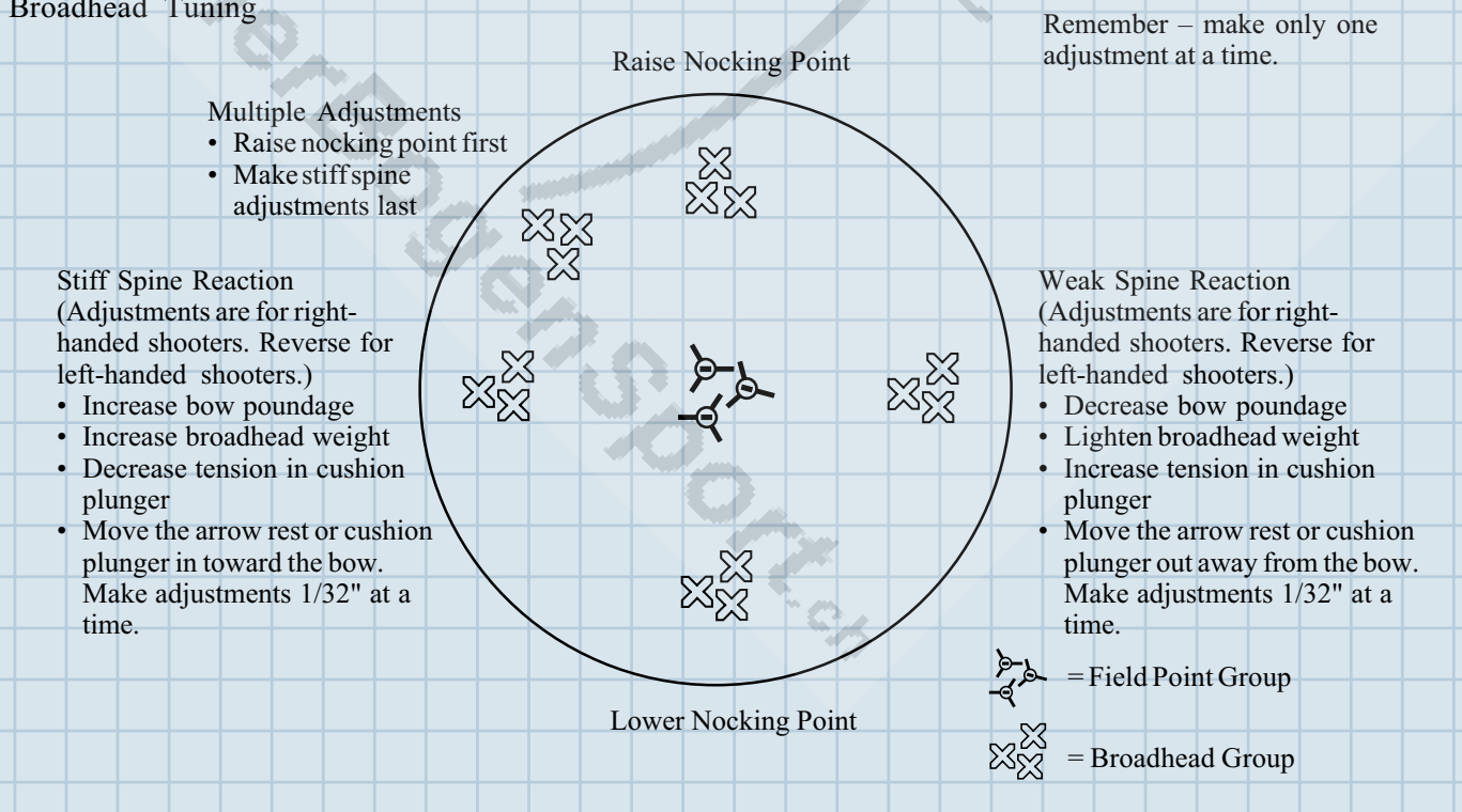
Fig. 20 Broadhead Tuning
